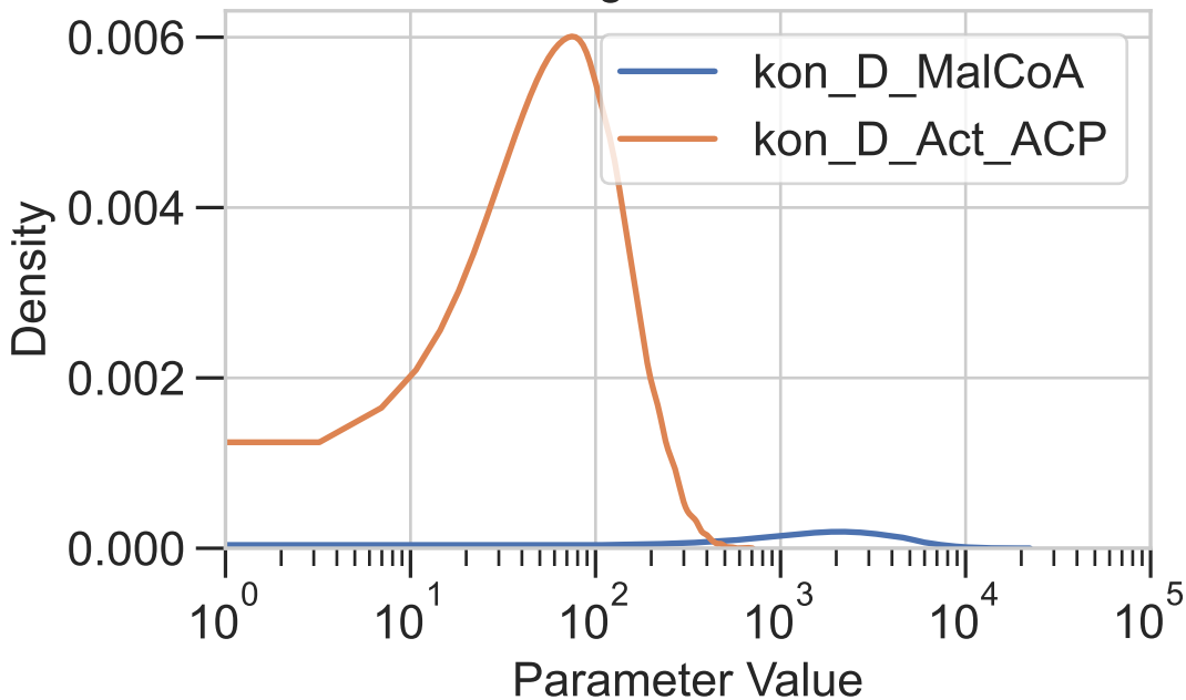
Prior Marginal Distributions
